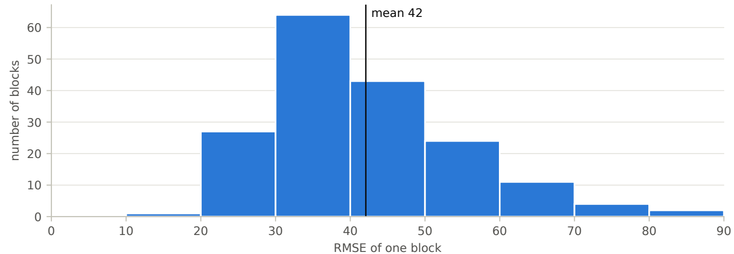
RMSE of each of the 176 validation blocks of 168 steps (submitted model)
